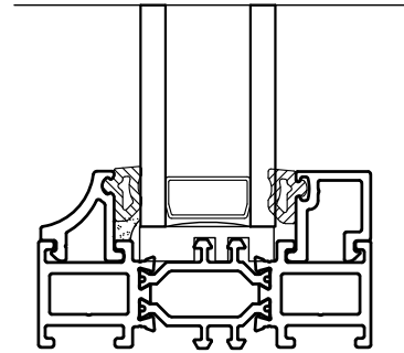
COVERED STOP OPTION
