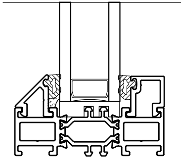
BEVELED STOP OPTION
