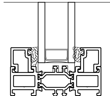
SQUARE STOP OPTION
