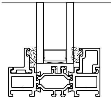
SETBACK LEG STOP OPTION
