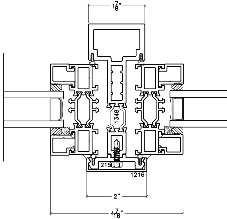
HEAVY 3-PIECE MULLION HORIZONTAL OR VERTICAL
