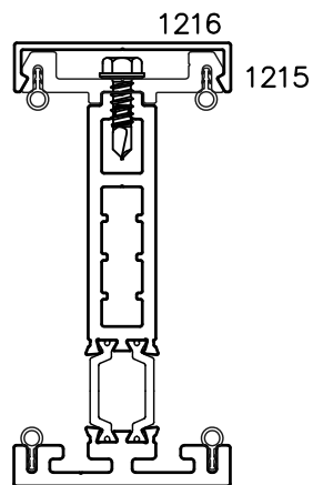
3-PIECE MULLION HORIZONTAL OR VERTICAL
