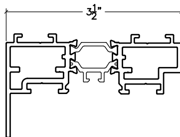
FIXED FRAME
