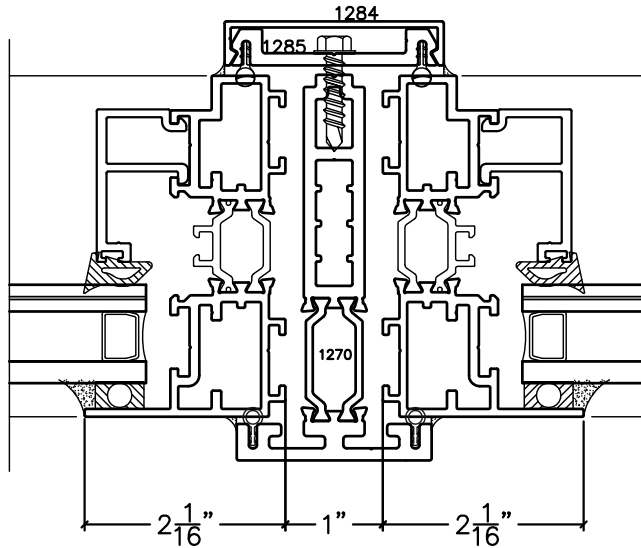
3 PC. MULLION HORIZONTAL OR VERTICAL
