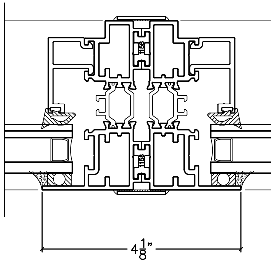
H-BAR MULLION HORIZONTAL OR VERTICAL
