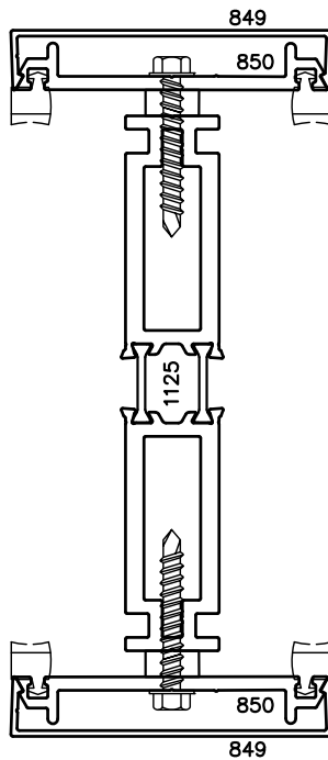
3 PC. MULLION HORIZONTAL OR VERTICAL
