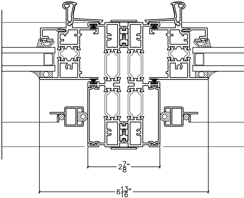
H-BAR MULLION HORIZONTAL OR VERTICAL
