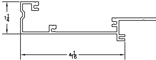
SCW-1102 MATES WITH SCW-1104 @ SILL
