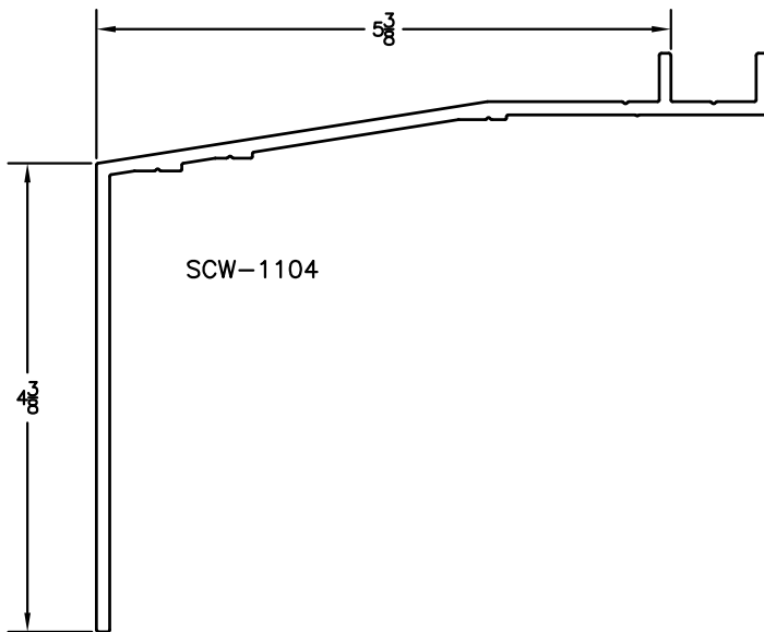
SCW-1103 MATES WITH SCW-1104 @ SILL
