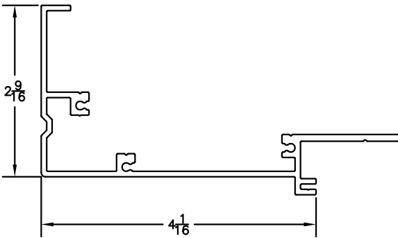
SCW-1103 MATES WITH SCW-1104 @ SILL
