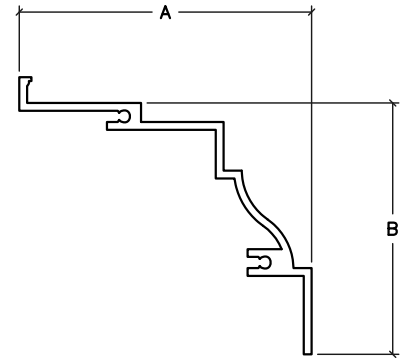
HEAD & JAMB CUSTOM OPTION
