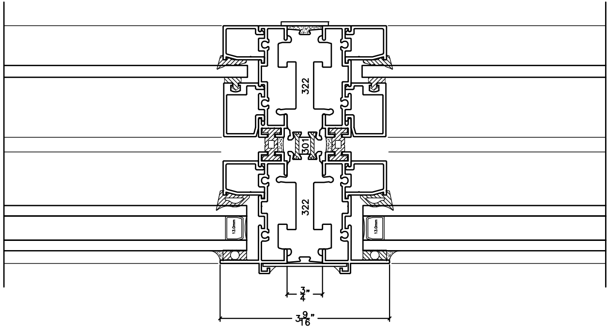
IMPACT MULLION HORIZONTAL OR VERTICAL
