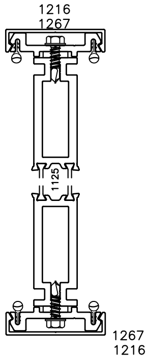
3-PIECE MULLION HORIZONTAL OR VERTICAL
