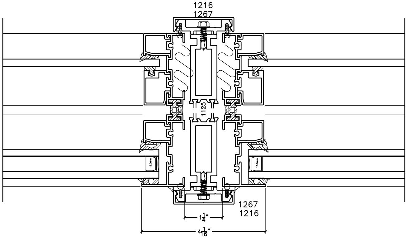
3-PIECE MULLION HORIZONTAL OR VERTICAL
